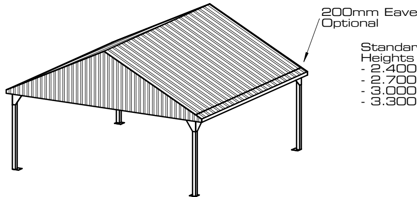
Gable Heritage Carport 26 deg Roof Pitch
