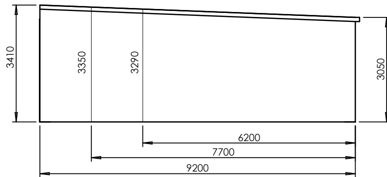
LOWLINE STANDARD SPANS AND HEIGHTS
