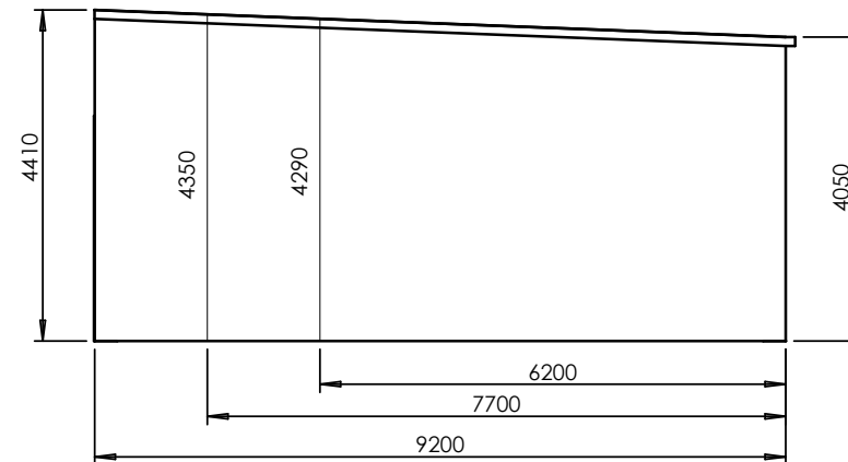
HIGHLINE STANDARD SPANS AND HEIGHTS
