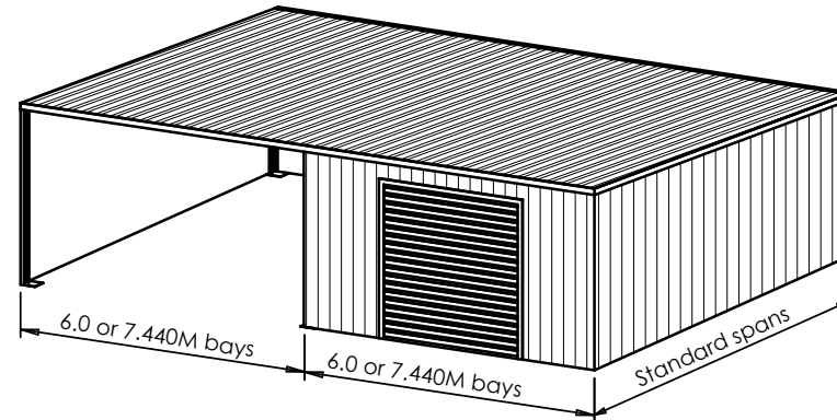
RURAL SKILLION GARAGES USE 6.0M OR 7.440M BAYS
