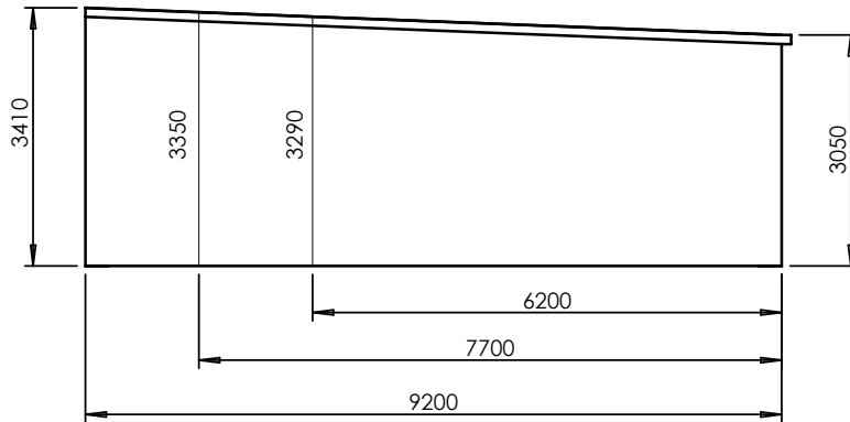
LOWLINE STANDARD SPANS AND HEIGHTS
