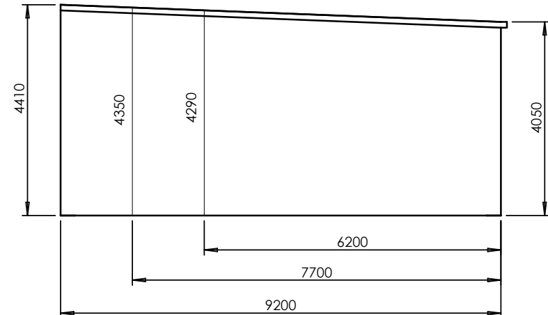
HIGHLINE STANDARD SPANS AND HEIGHTS
