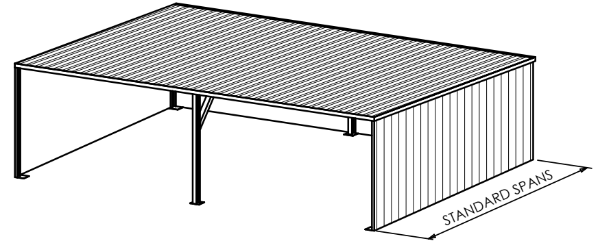
MULTIPLE BAY SKILLIONS USE 6.0M OR 7.440M BAYS TO CREATE 12M, 14.880, 18M, 22.320, GUTTER LENGTHS
